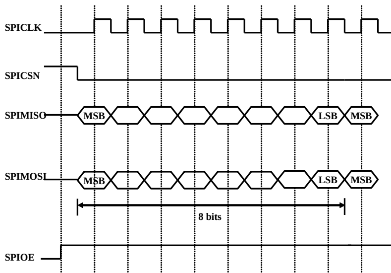
Figure43. Master Mode, SPO = 0, SPH=1
