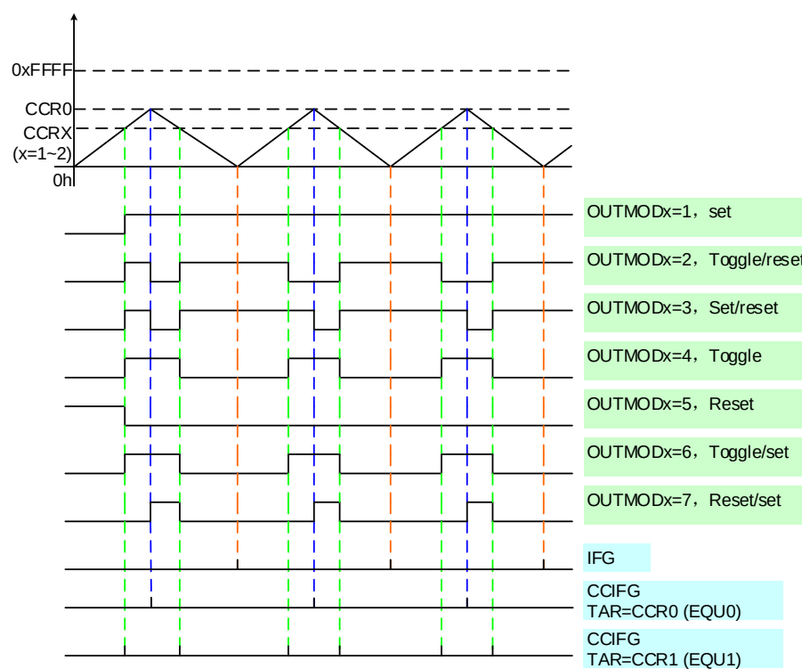
Figure33. PWM Output under Up/down Count Mode
