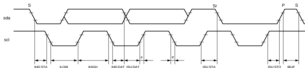
Figure54. AC Timing of I2C Controller
