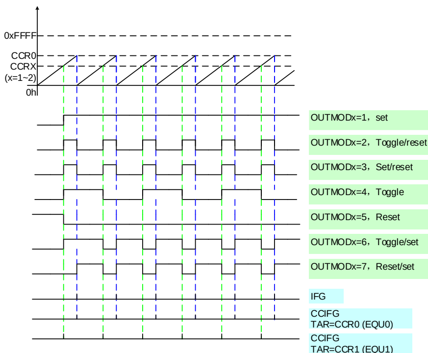
Figure31. PWM Output under Up-count Mode
