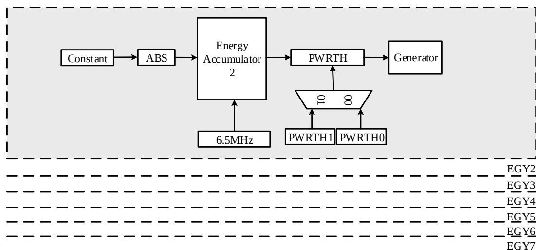
Figure63. Functional Block Diagram of low-speed energy accumulator
