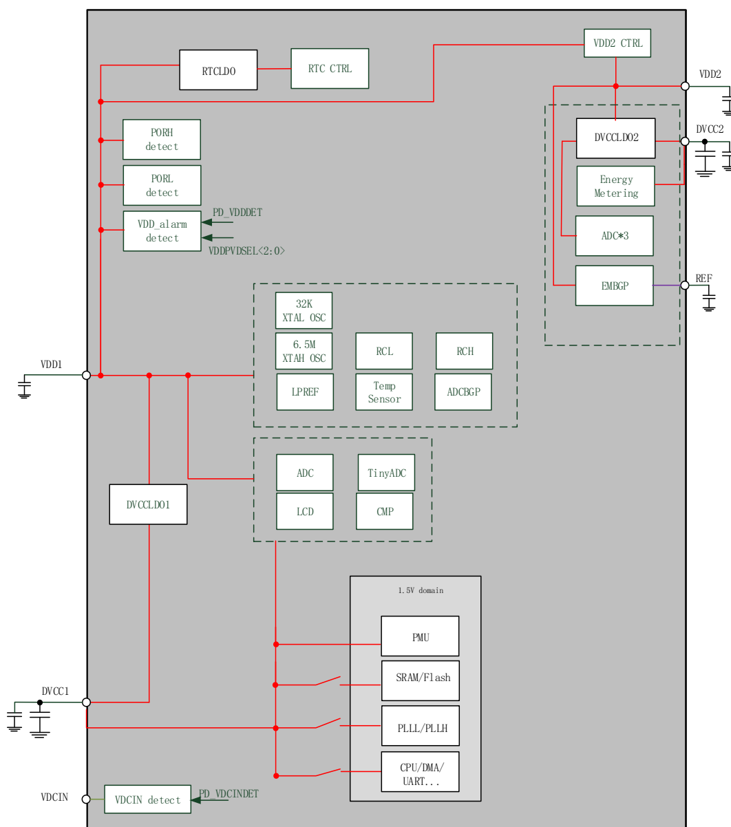
Figure5. V94XX Power System Block Diagram
