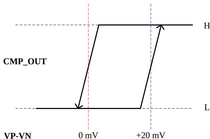
Figure17. hysteresis Window of CMP Controller
