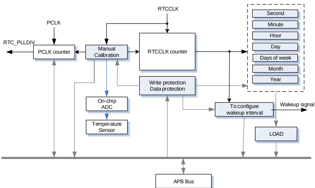
Figure19. Functional Block Diagram of RTC Controller
