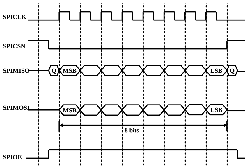
Figure43. Master Mode, SPO = 0, SPH=1
