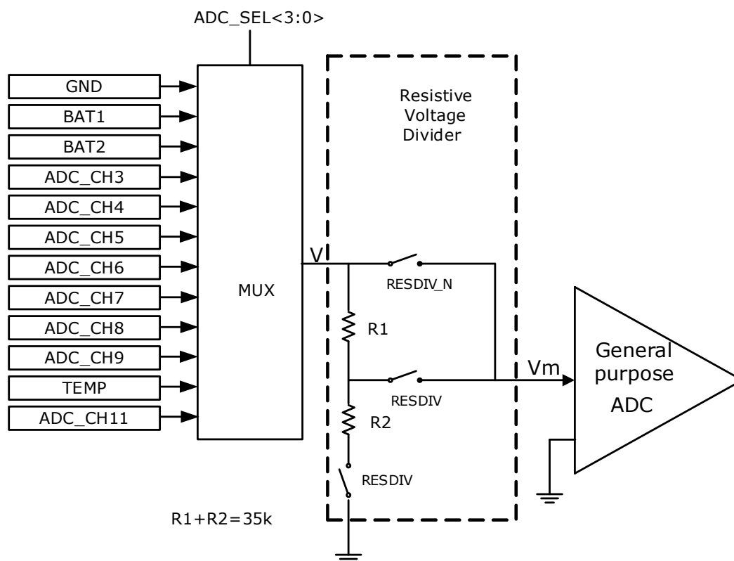
Figure16. ADC Architecture
