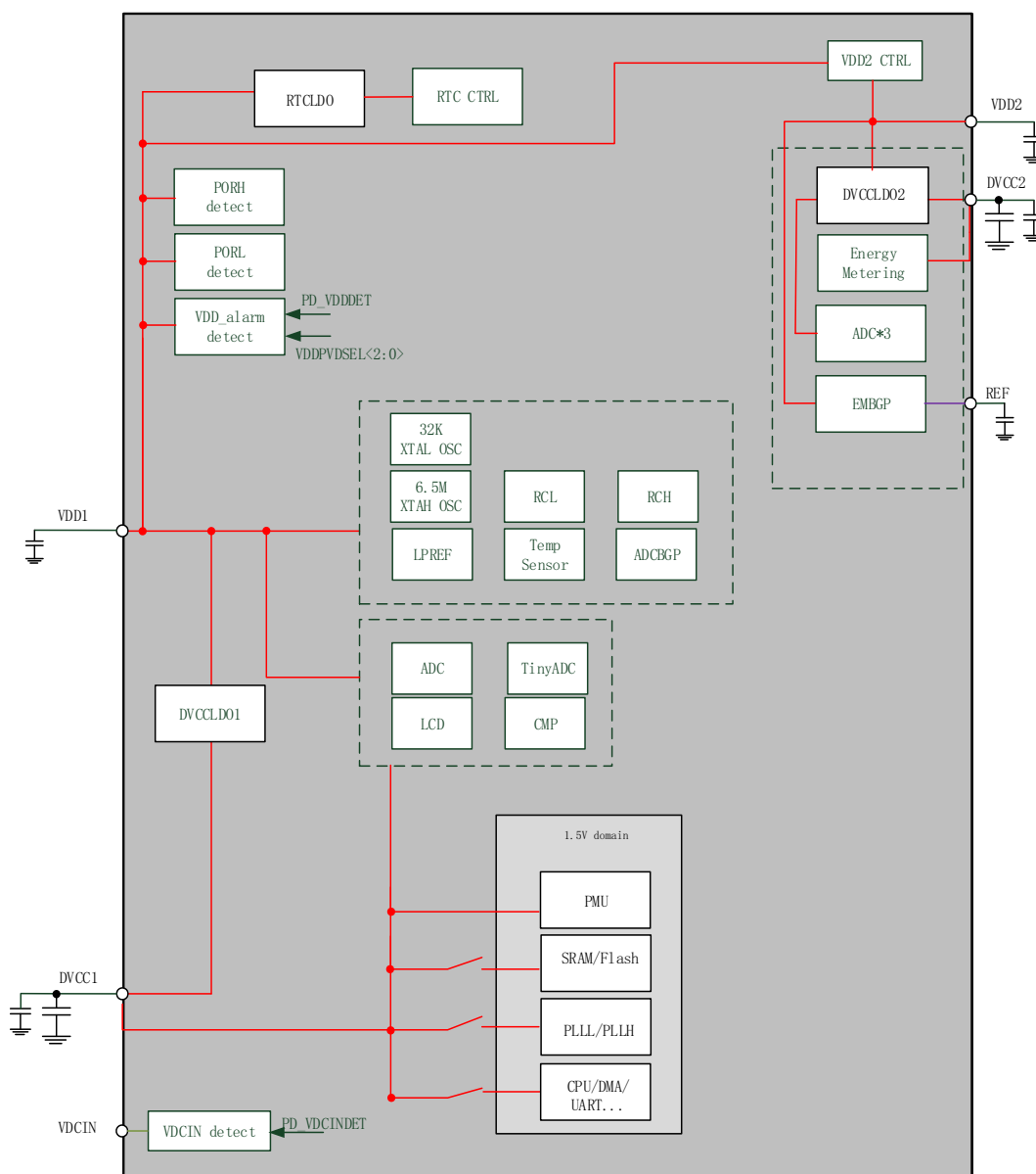
Figure2. V94XX Power System Block Diagram
