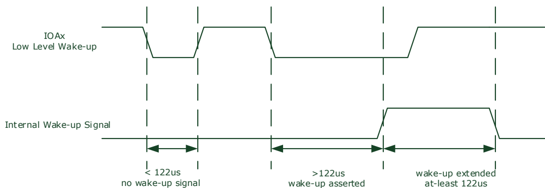
Figure11. External Wake-up Example
