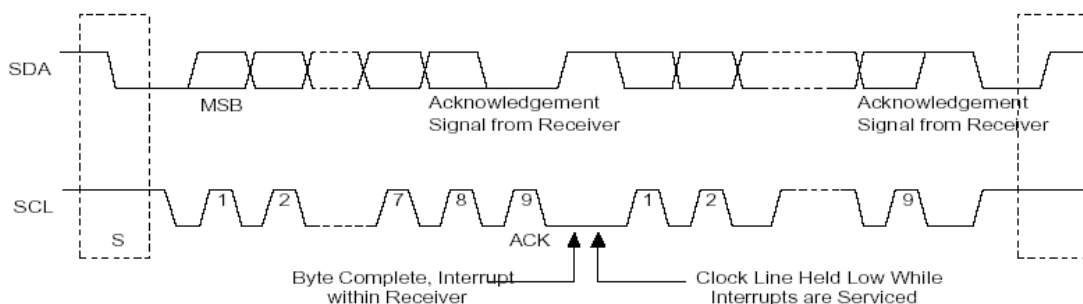
Figure50. Data Transfer on The I2C bus
