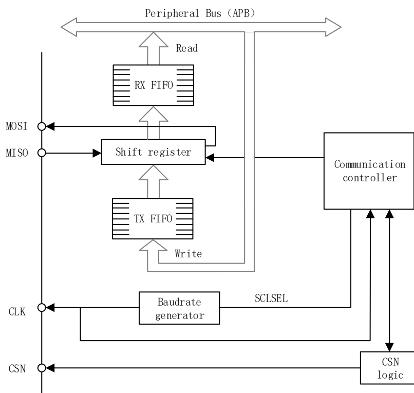
Figure41. Functional Block Diagram of SPI Controller
