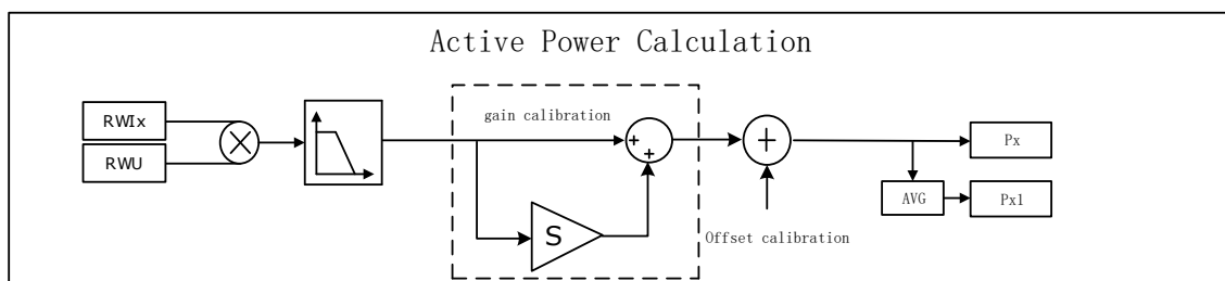
Figure73. Signal Processing for Active Power Calculation and Calibration
