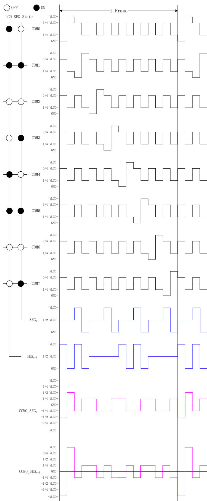
Figure39. LCD Drive Waveform of 1/8 Duty and 1/4 Bias
