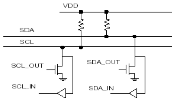
Figure52. I2C Bus Connection Example
