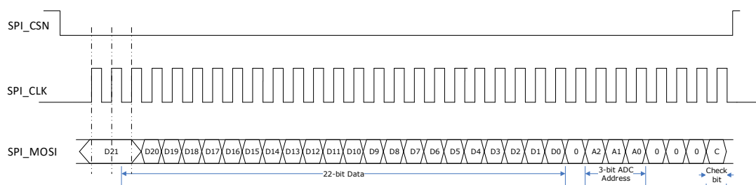
Figure77. Communication timing of SPI
