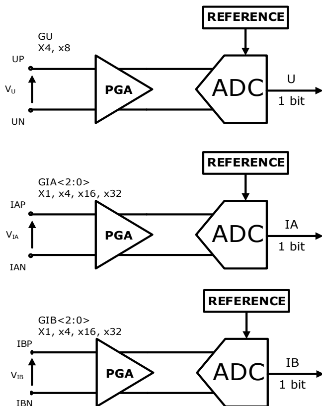
Figure69. Current/voltage channel analog gain configuration
