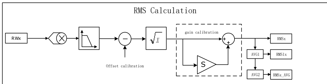
Figure72. RMS Calculation and Calibration
