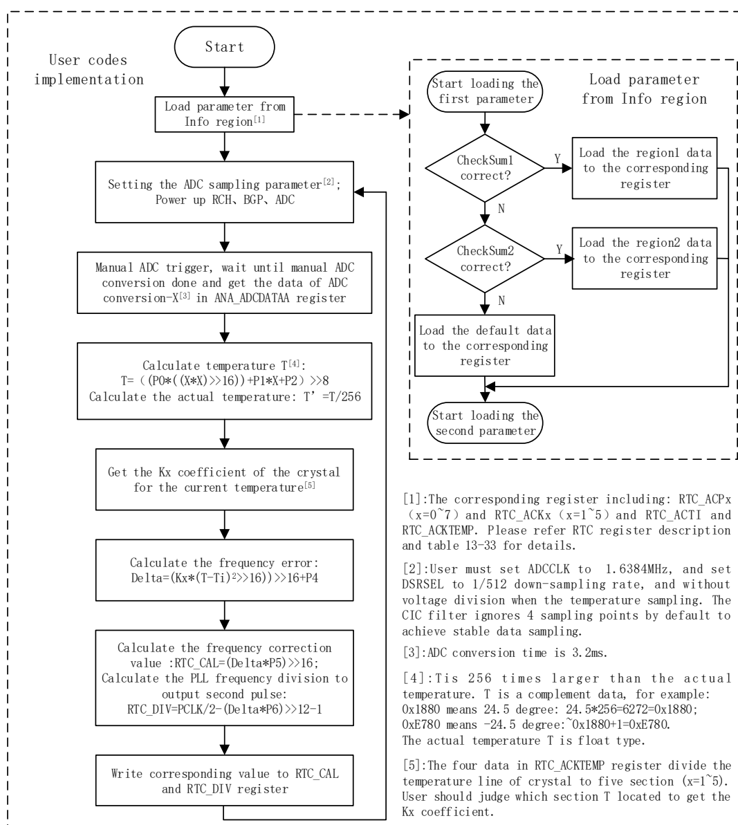
Figure20. RTC Manual Temperature Compensation Flow Chart
