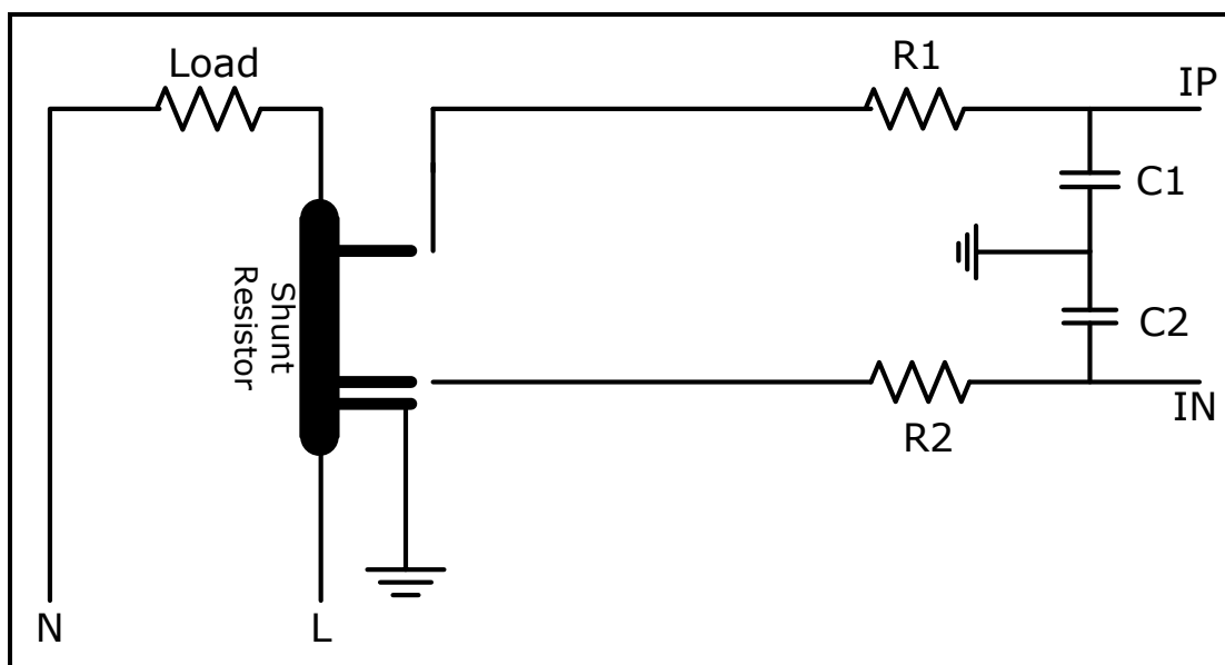
Figure67. Shunt Resistor Network for Current Analog Input
