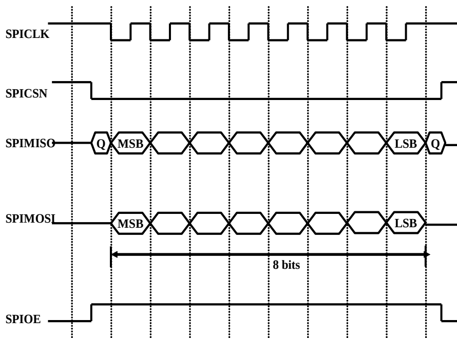
Figure45. Master Mode, SPO = 1, SPH=1
