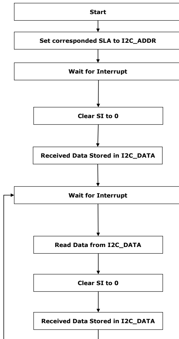
Figure58. Operations for Slave Receiver Mode
