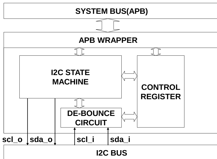
Figure46. Functional Block Diagram of I2C Controller
