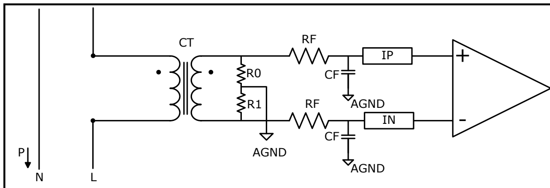
Figure66. CT for Current Analog Input
