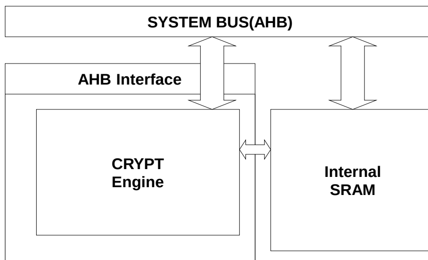
Figure60. Functional Block Diagram of CRYPT Controller
