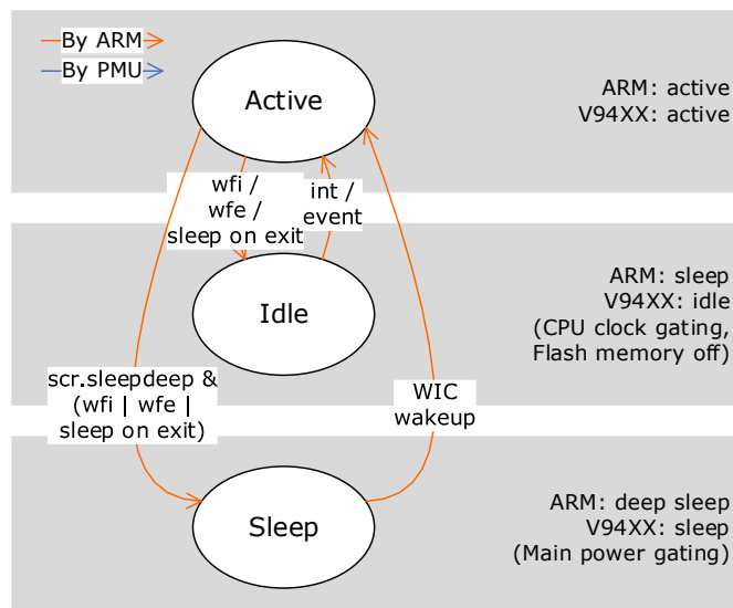
Figure10. Power State Flow Chart of V94XX
