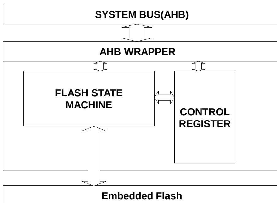
Figure21. Functional Block Diagram of FLASH Controller
