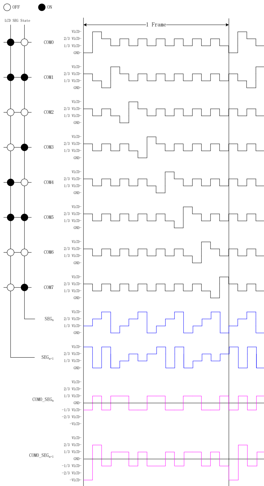
Figure38. LCD Drive Waveform of 1/8 Duty and 1/3 Bias
