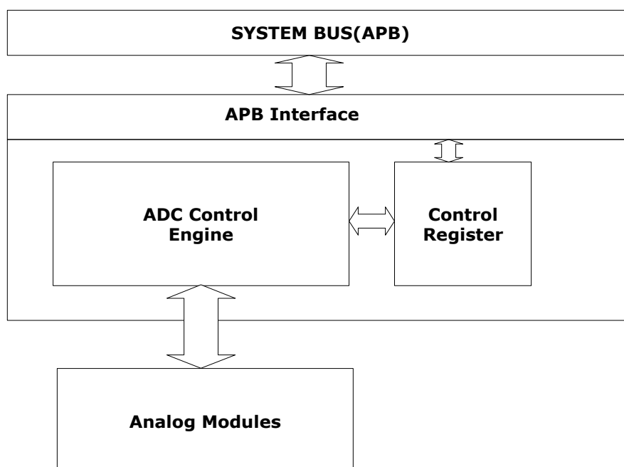
Figure15. Functional Block Diagram of Analog Controller
