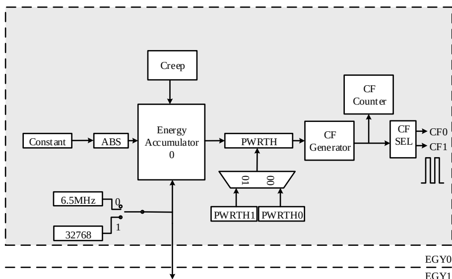
Figure63. Functional Block Diagram of low-speed energy accumulator
