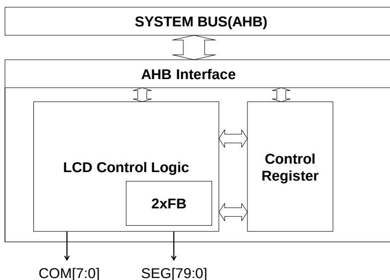
Figure34. Functional Block Diagram of LCD Controller
