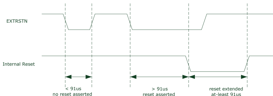
Figure9. External Reset De-glitch Timing
