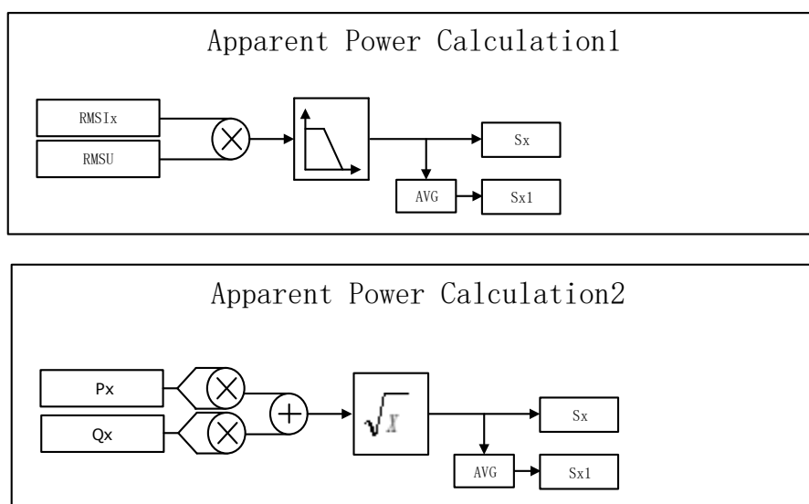
Figure75. Apparent Power Calculation
