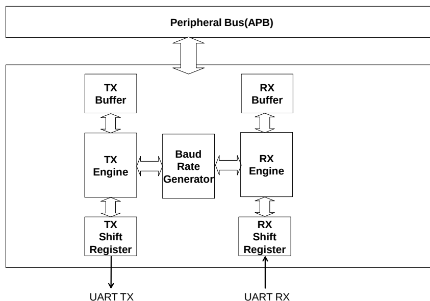
Figure24. Functional Block Diagram of UART Controller
