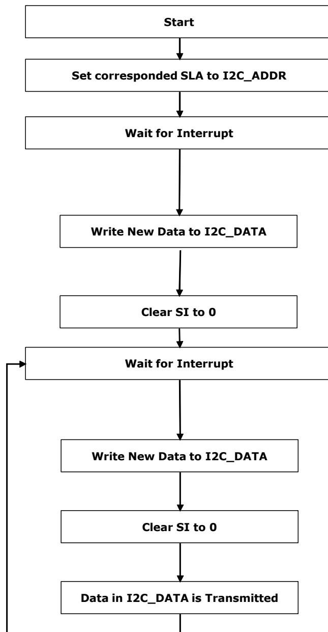
Figure57. Operations for Slave Transmitter Mode
