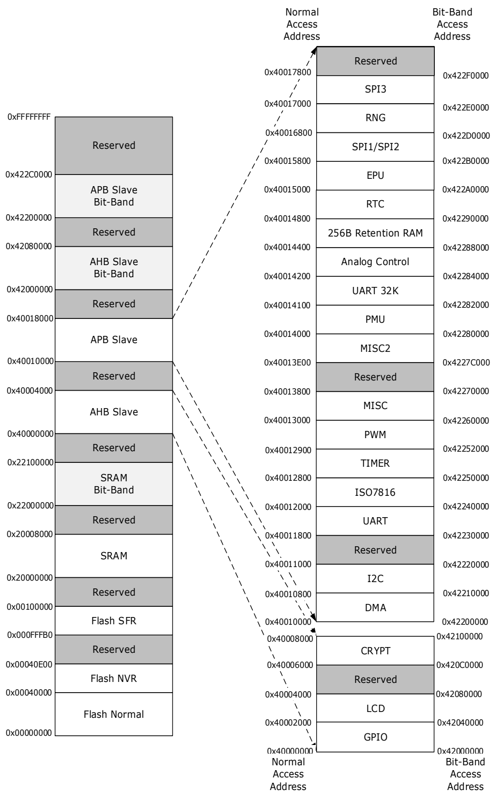
Figure4. V94XX Memory Maps
