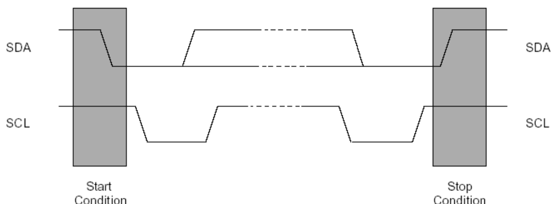
Figure47. Start and Stop Conditions
