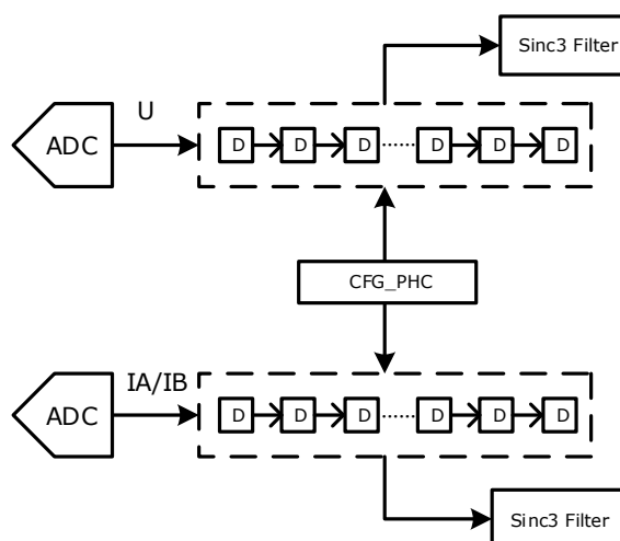
Figure70. Phase Compensation Schematics
