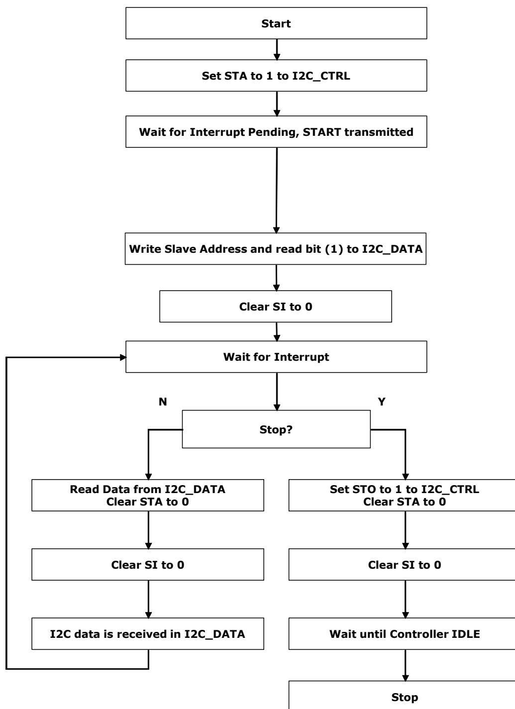
Figure56. Operations for Master Receiver Mode
