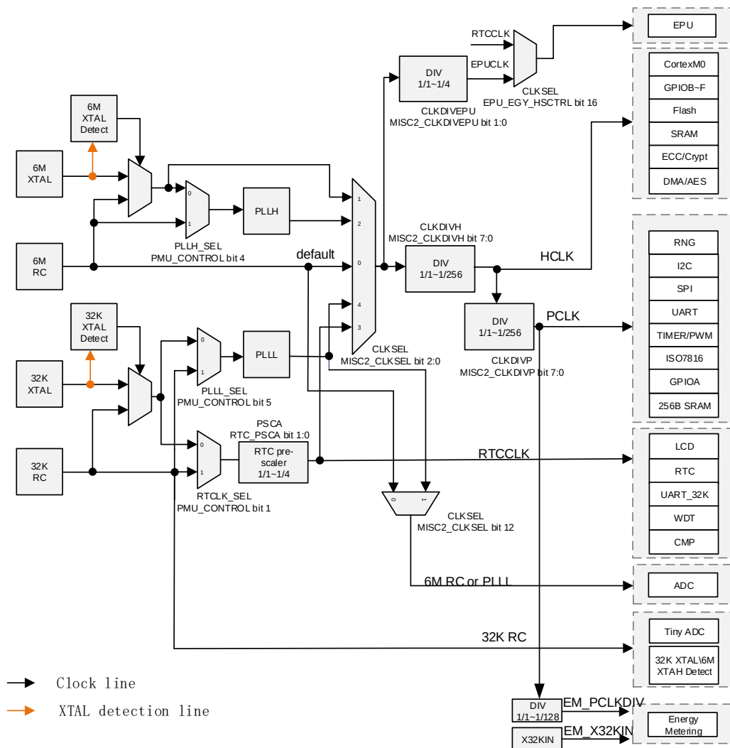
Figure3. V94XX Clock Block Diagram
