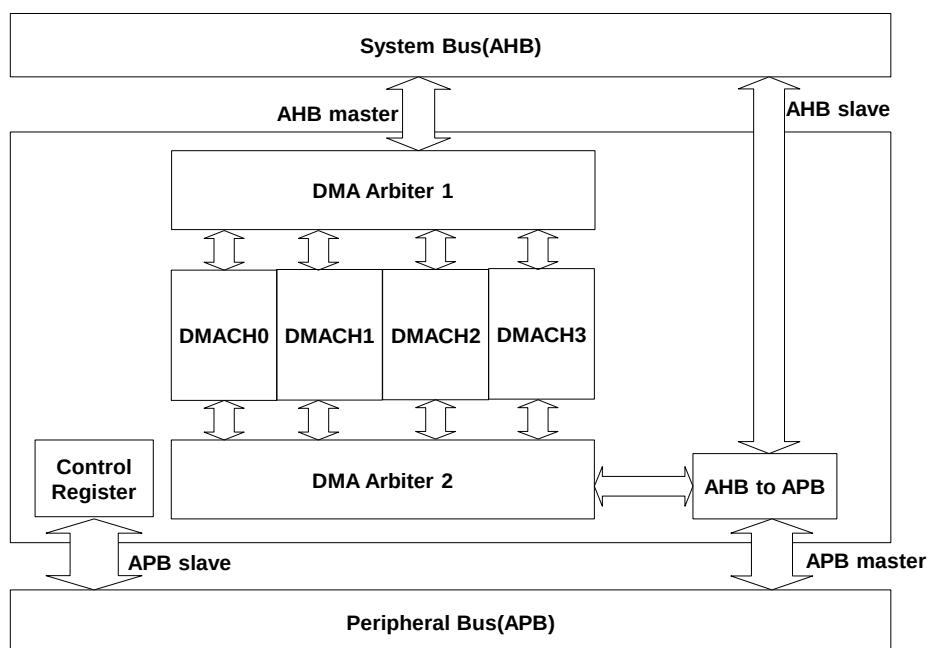
Figure23. Functional Block Diagram of DMA Controller
