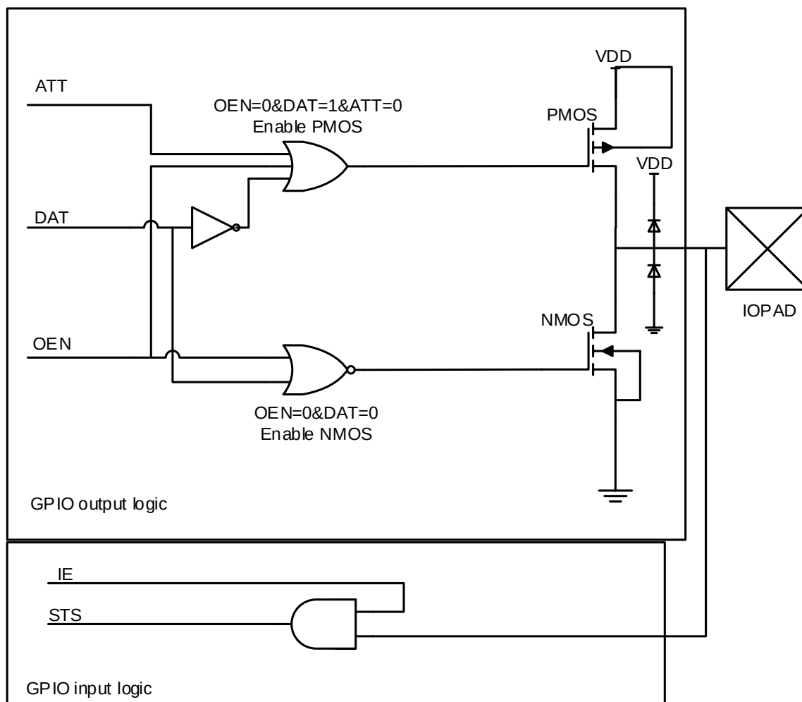
Figure22. Functional Block Diagram of GPIO Controller
