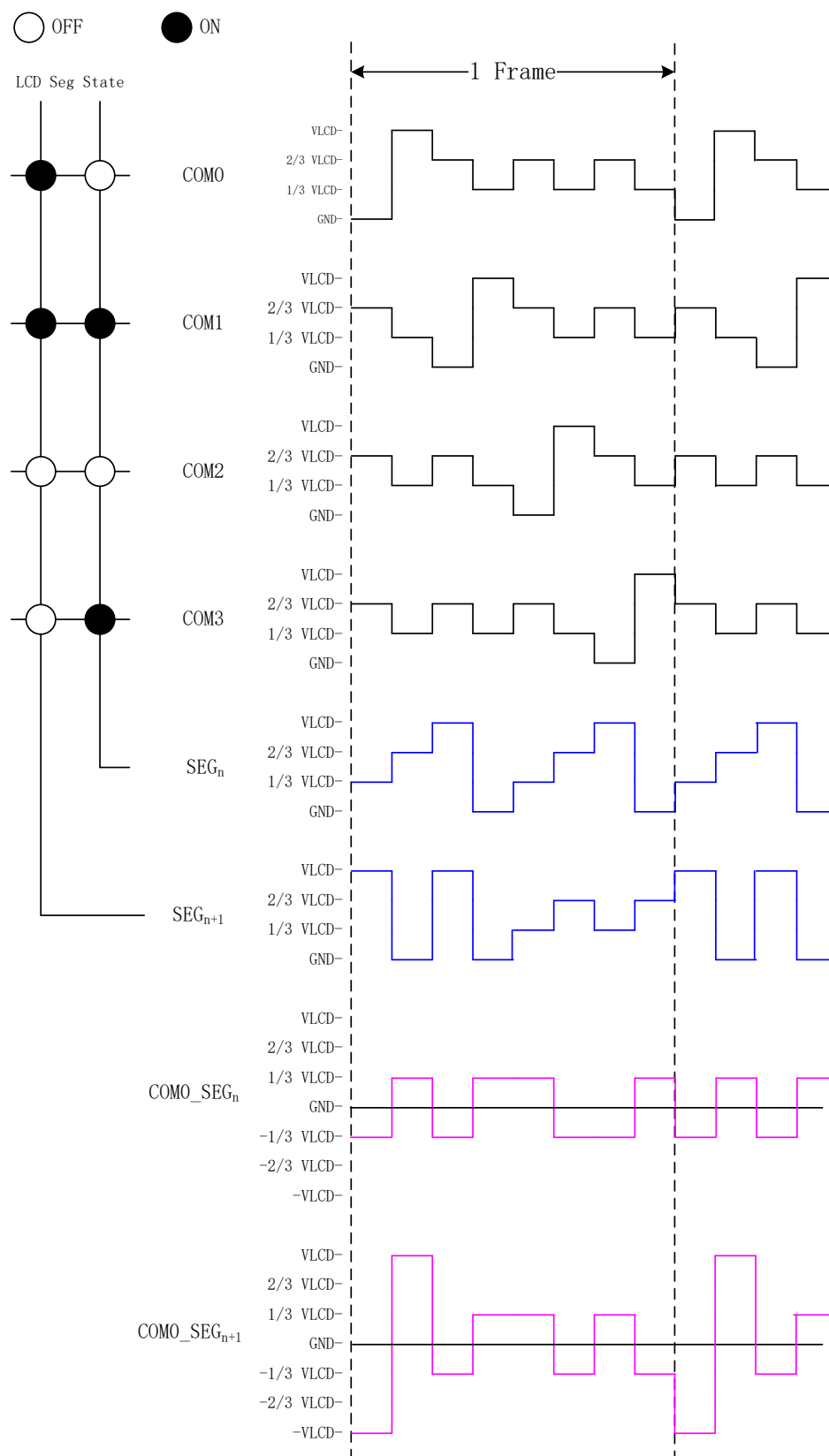
Figure36. LCD Drive Waveform of 1/4 Duty and 1/3 Bias
