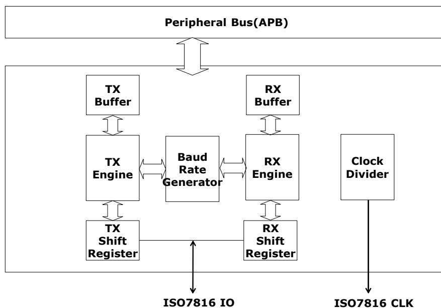
Figure26. Functional Block Diagram of ISO7816 Controller
