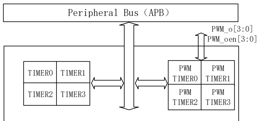
Figure28. Functional Block Diagram of PWM TIMER Controller
