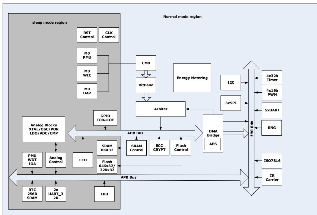
Figure1. V94XX Functional Block Diagram
