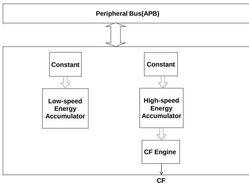
Figure61. Functional Block Diagram of EPU Controller
