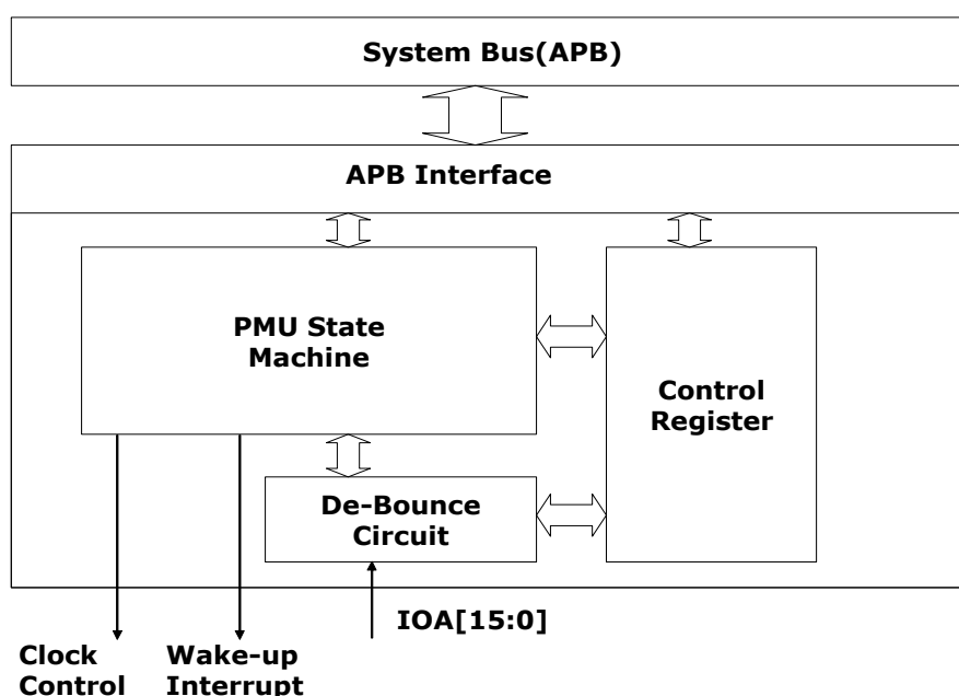
Figure8. Functional Block Diagram of PMU Controller
