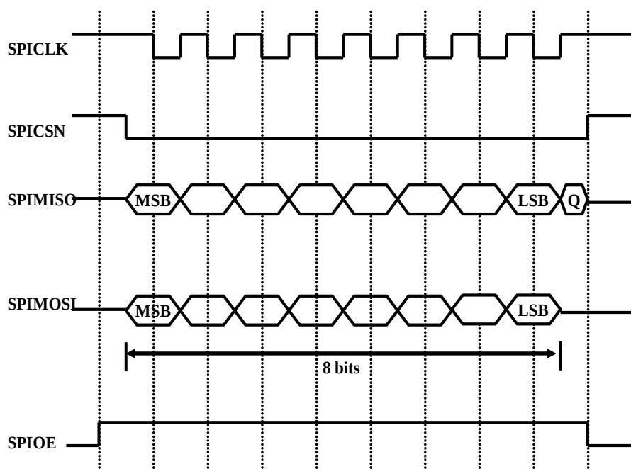
Figure45. Master Mode, SPO = 1, SPH=1
