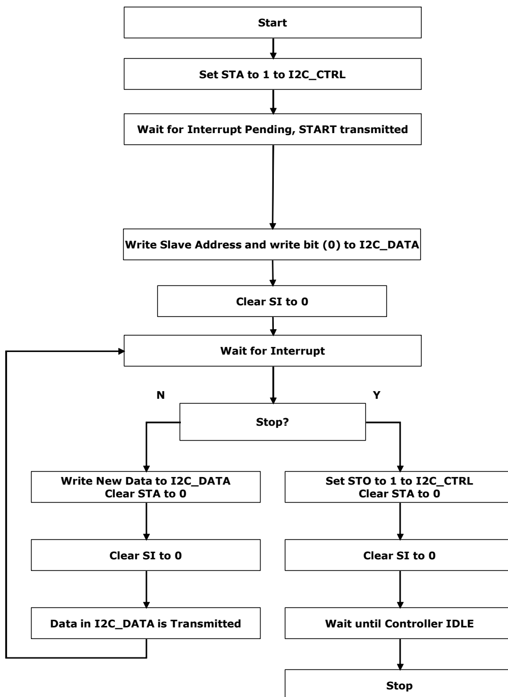
Figure55. Operations for Master Transmitter Mode
