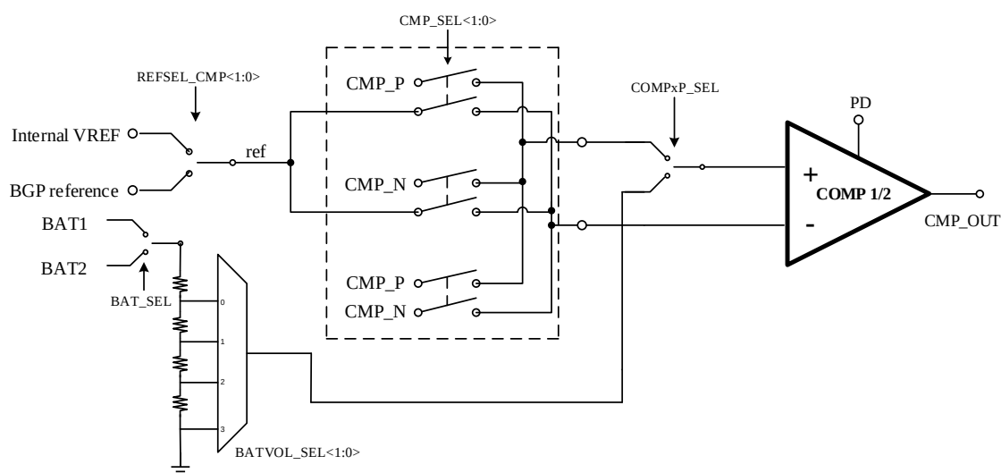
Figure18. Functional Block Diagram of CMP Controller
