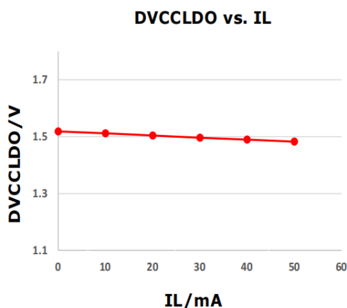
Figure6. DVCC1DO Output and The Load Current Power Supply Supervisor
