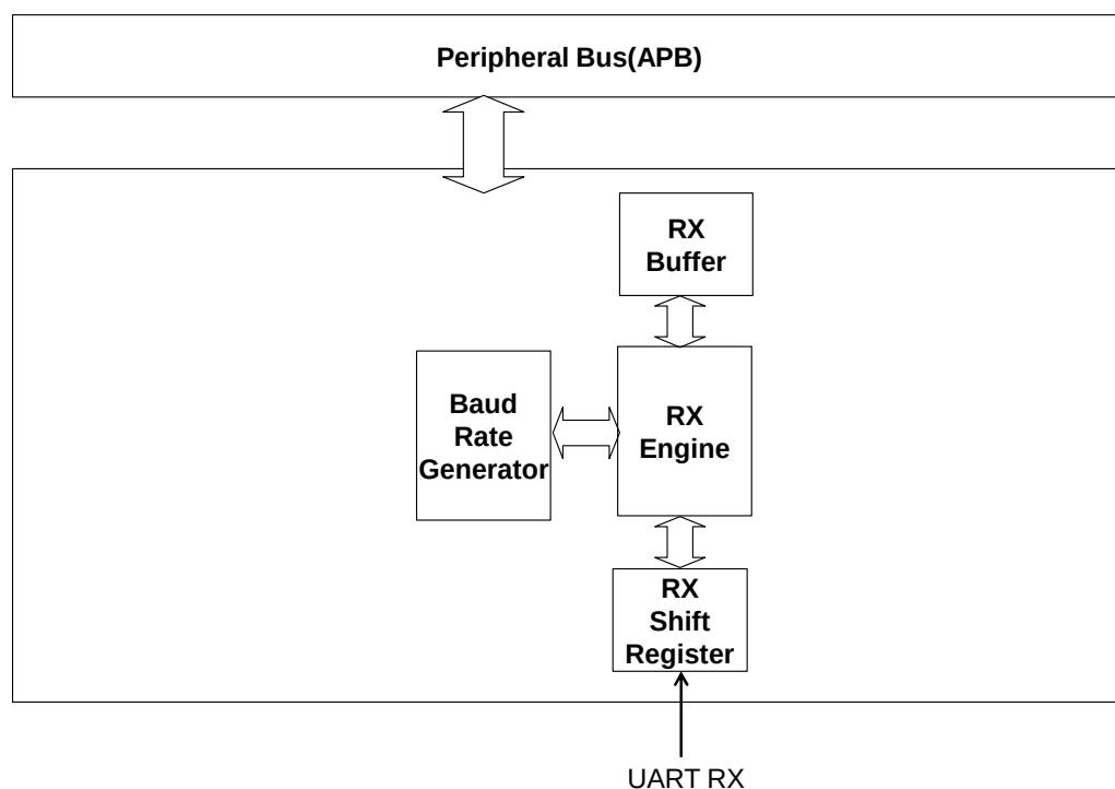
Figure25. Functional Block Diagram of UART 32K Controller
