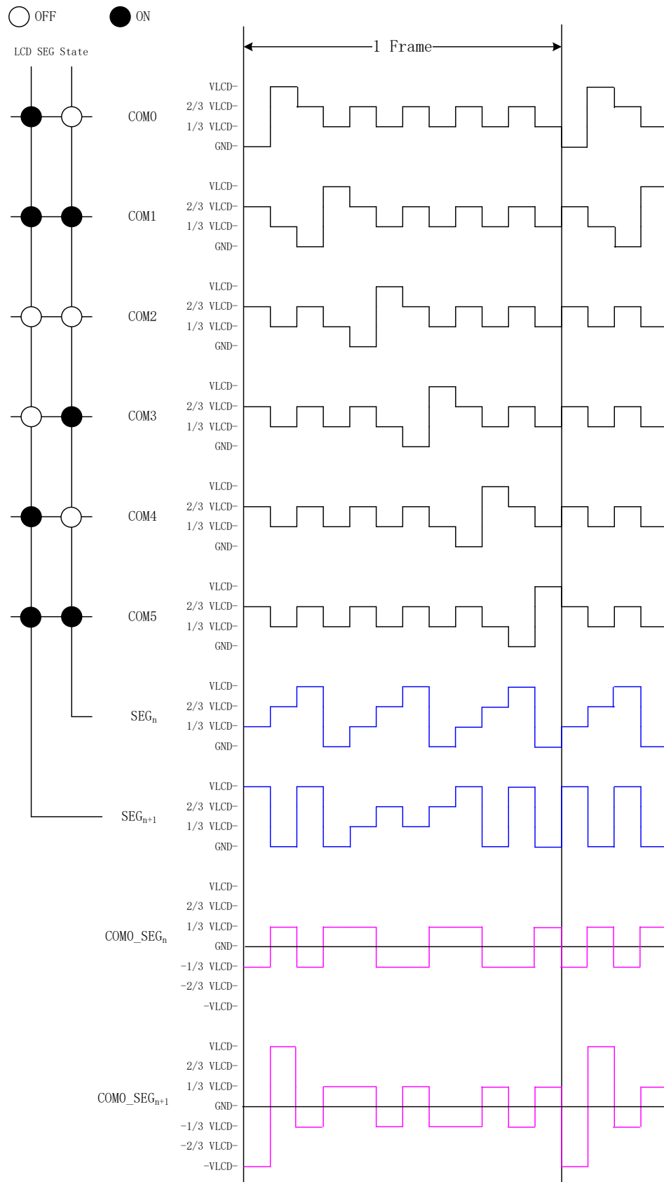
Figure37. LCD Drive Waveform of 1/6 Duty and 1/3 Bias
