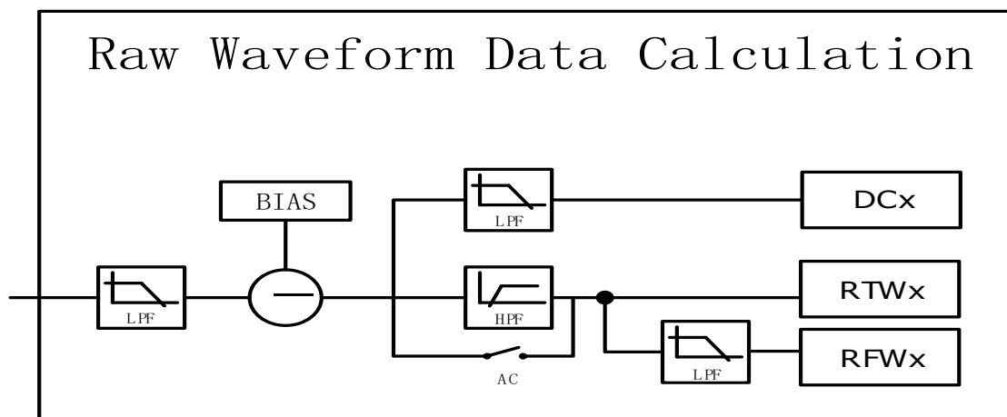
Figure71. Generation of raw waveform data
