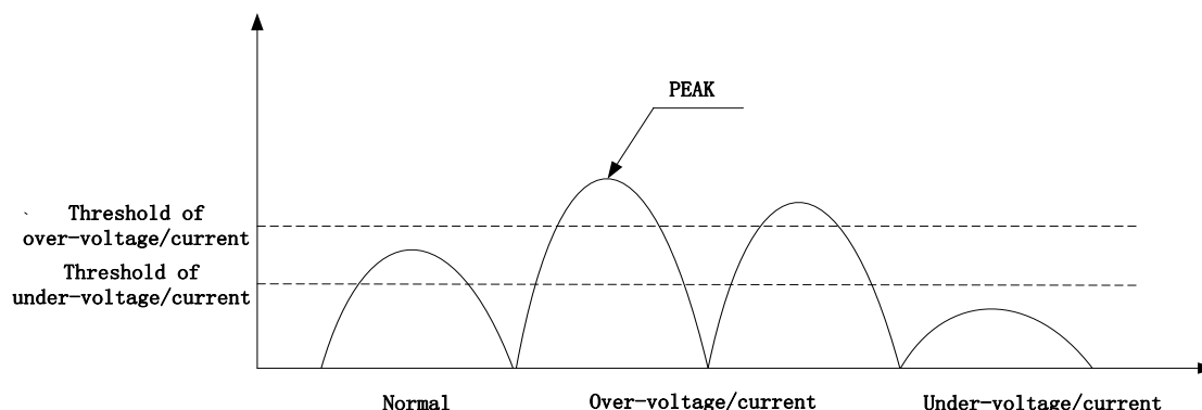
Figure79. Over-voltage and under-voltage/Over-current and under-current detect
