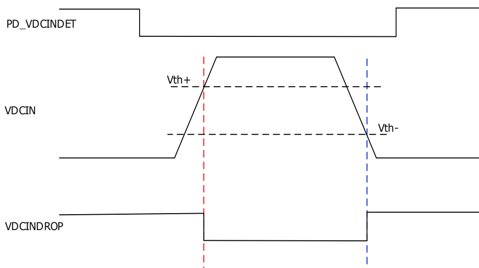
Figure7. Relation Between VDCIN Input Signal and States of Flag Bits VDCINDROP
