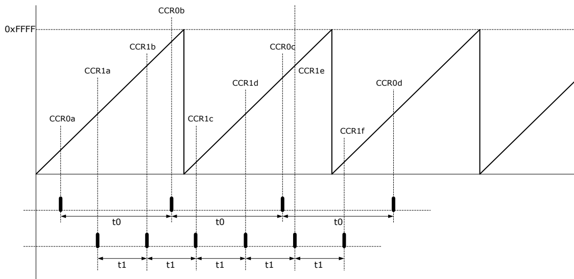
Figure30. Example of Continuous Mode
