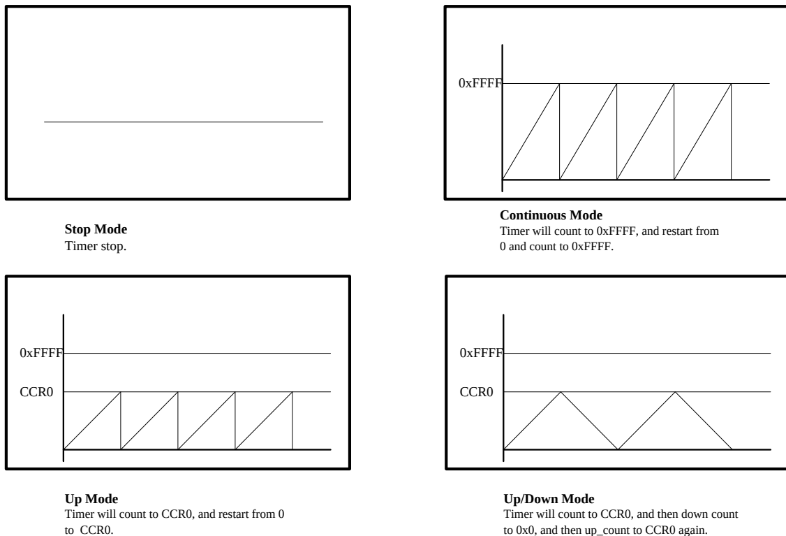
Figure29. Mode description of PWM TIMER Controller
