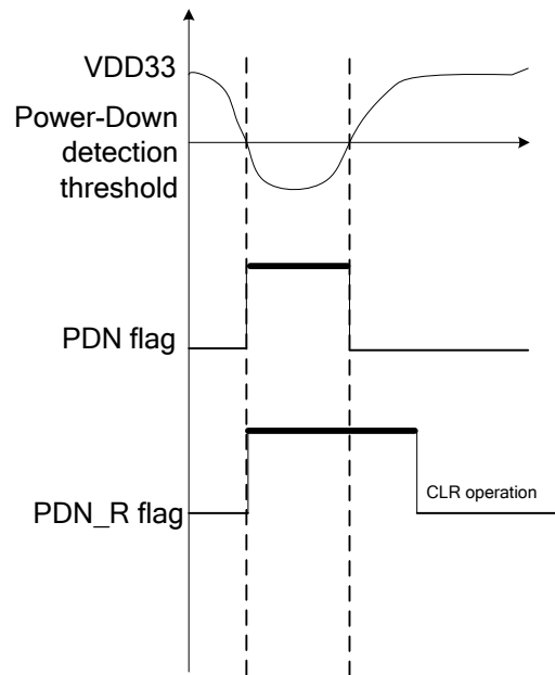
Figure 4-2 Power-Down Interrupt
