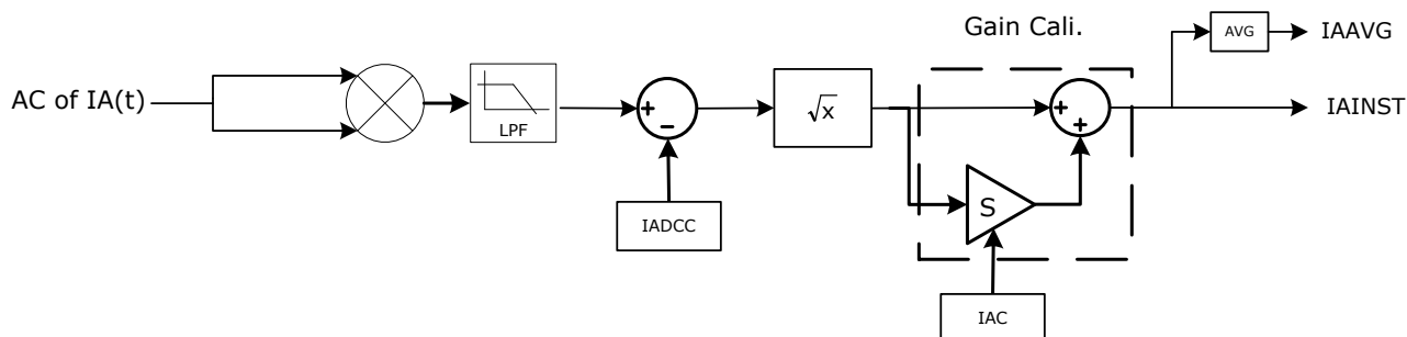
Figure 7-5 RMS Signal Processing
