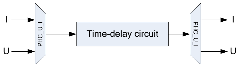
Figure 7-3 Phase Compensation
