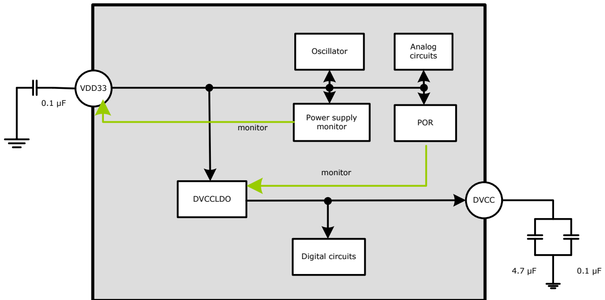
Figure 4-1 Power Supply Architecture
