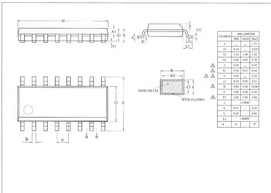
Figure13. Outline dimension for V9160
