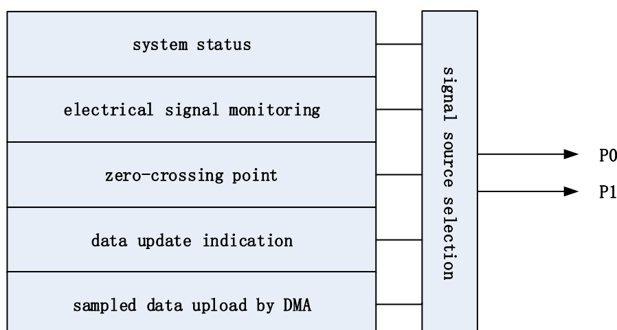
Figure12. Functional Block Diagram of Signal Output Port
