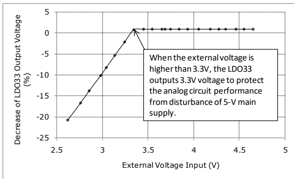
Figure 8-2 LDO33 Output and 5V Power Input
