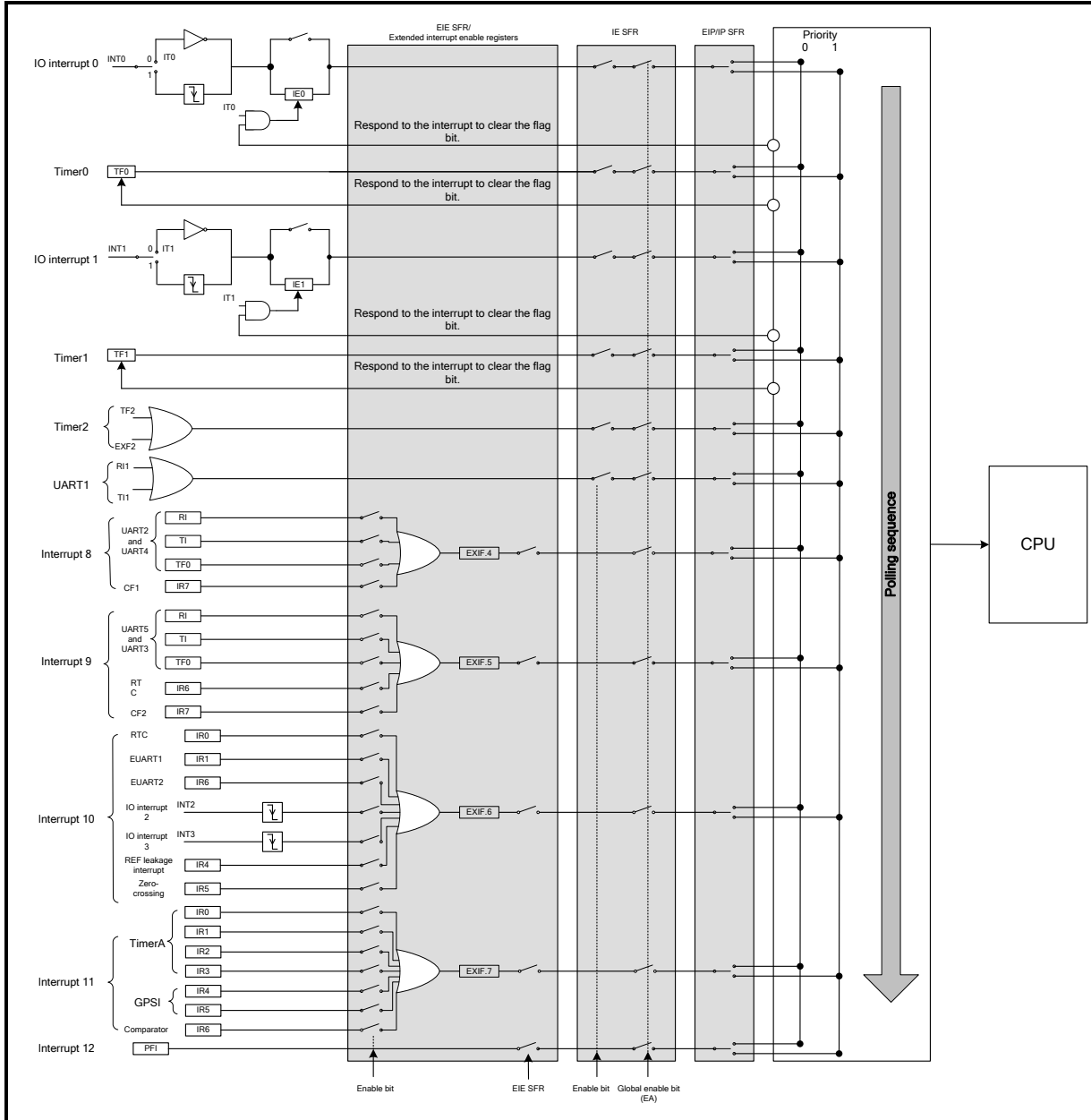
Figure 11-1 Interrupt Logic
