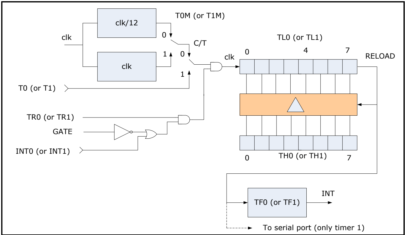
Figure 12-8 Timer 0/1, Mode 2
